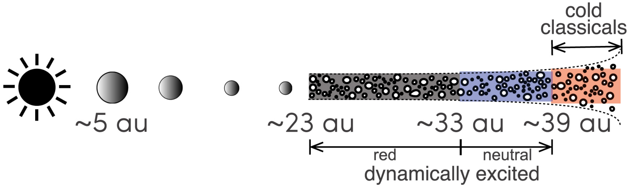
Figure 6. from Col-OSSOS: The Colors of the Outer Solar System Origins Survey null 2019 APJS 243 12 doi:10.3847/1538-4365/ab2194 http://dx.doi.org/10.3847/1538-4365/ab2194 © 2019. The American Astronomical Society. All rights reserved.
