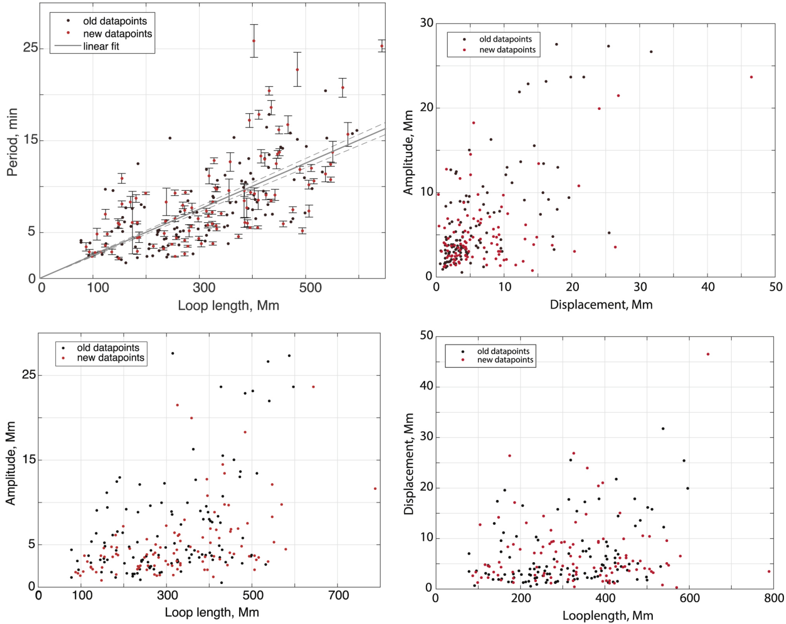
Figure 5. from Catalog of Decaying Kink Oscillations of Coronal Loops in the 24th Solar Cycle null 2019 APJS 241 31 doi:10.3847/1538-4365/ab0e86 http://dx.doi.org/10.3847/1538-4365/ab0e86 © 2019. The American Astronomical Society. All rights reserved.
