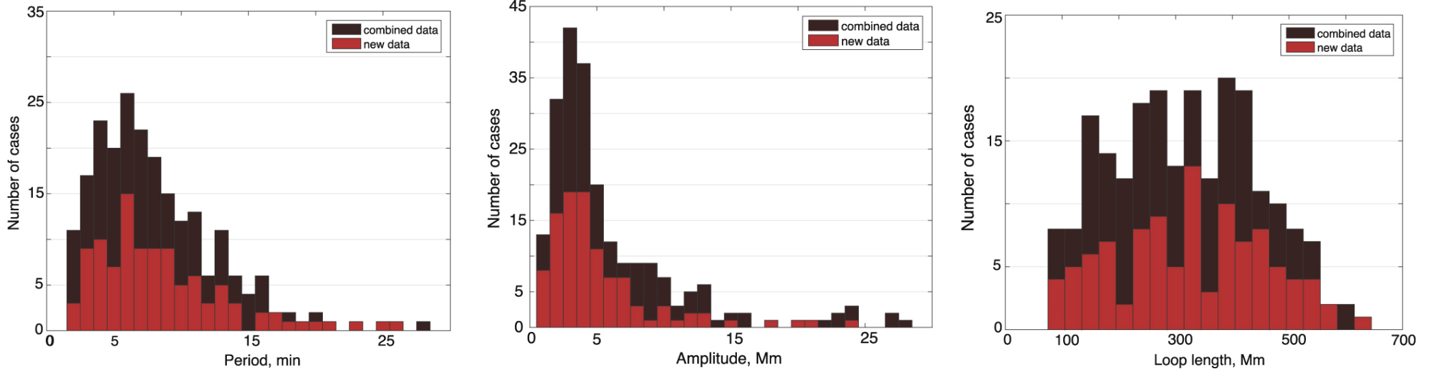
Figure 4. from Catalog of Decaying Kink Oscillations of Coronal Loops in the 24th Solar Cycle null 2019 APJS 241 31 doi:10.3847/1538-4365/ab0e86 http://dx.doi.org/10.3847/1538-4365/ab0e86
