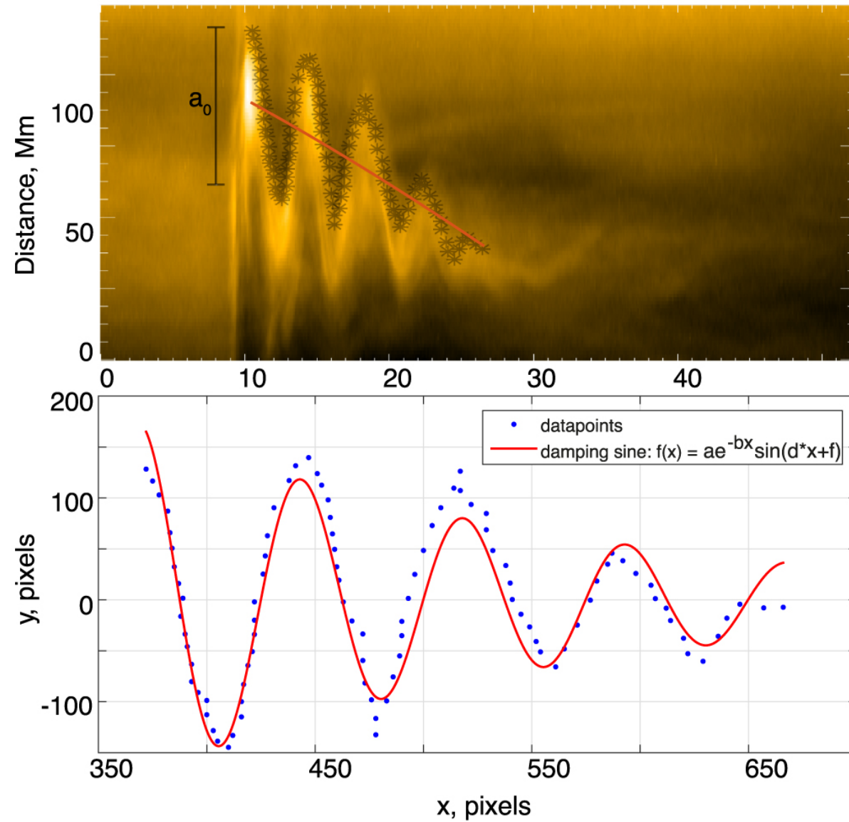
Figure 3. from Catalog of Decaying Kink Oscillations of Coronal Loops in the 24th Solar Cycle null 2019 APJS 241 31 doi:10.3847/1538-4365/ab0e86 http://dx.doi.org/10.3847/1538-4365/ab0e86 © 2019. The American Astronomical Society. All rights reserved.
