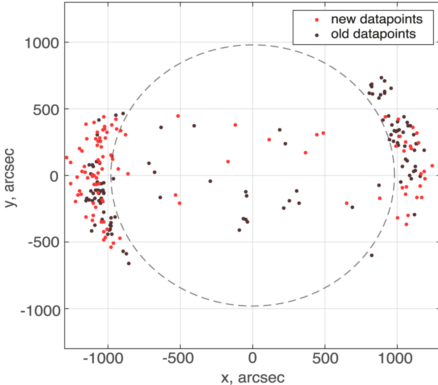
Figure 2. from Catalog of Decaying Kink Oscillations of Coronal Loops in the 24th Solar Cycle null 2019 APJS 241 31 doi:10.3847/1538-4365/ab0e86 http://dx.doi.org/10.3847/1538-4365/ab0e86 © 2019. The American Astronomical Society. All rights reserved.
