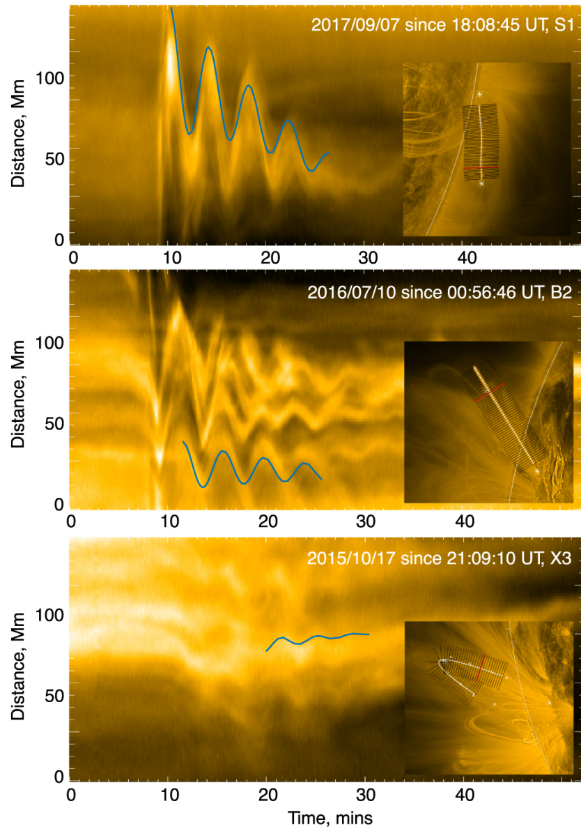
Figure 1. from Catalog of Decaying Kink Oscillations of Coronal Loops in the 24th Solar Cycle null 2019 APJS 241 31 doi:10.3847/1538-4365/ab0e86 https://dx.doi.org/10.3847/1538-4365/ab0e86 © 2019. The American Astronomical Society. All rights reserved.
