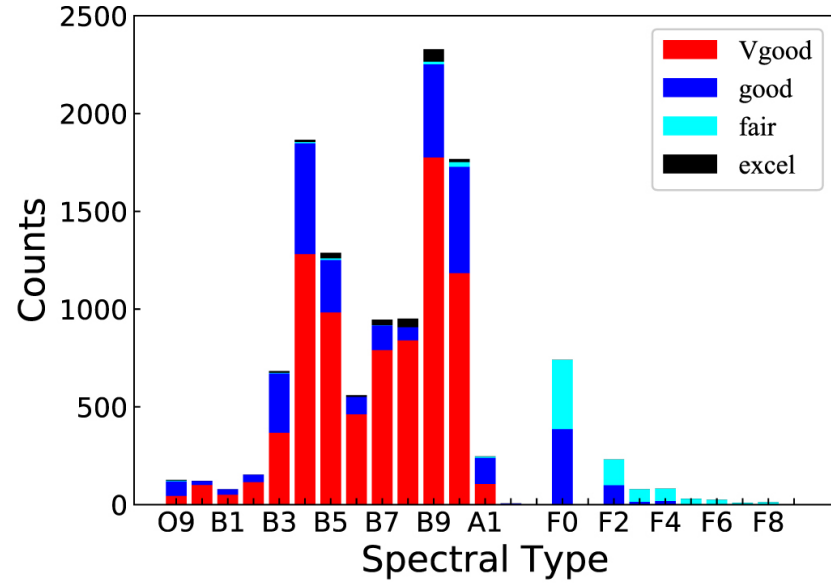
Figure 9. from A Catalog of OB Stars from LAMOST Spectroscopic Survey null 2019 APJS 241 32 doi:10.3847/1538-4365/ab0a0d http://dx.doi.org/10.3847/1538-4365/ab0a0d
