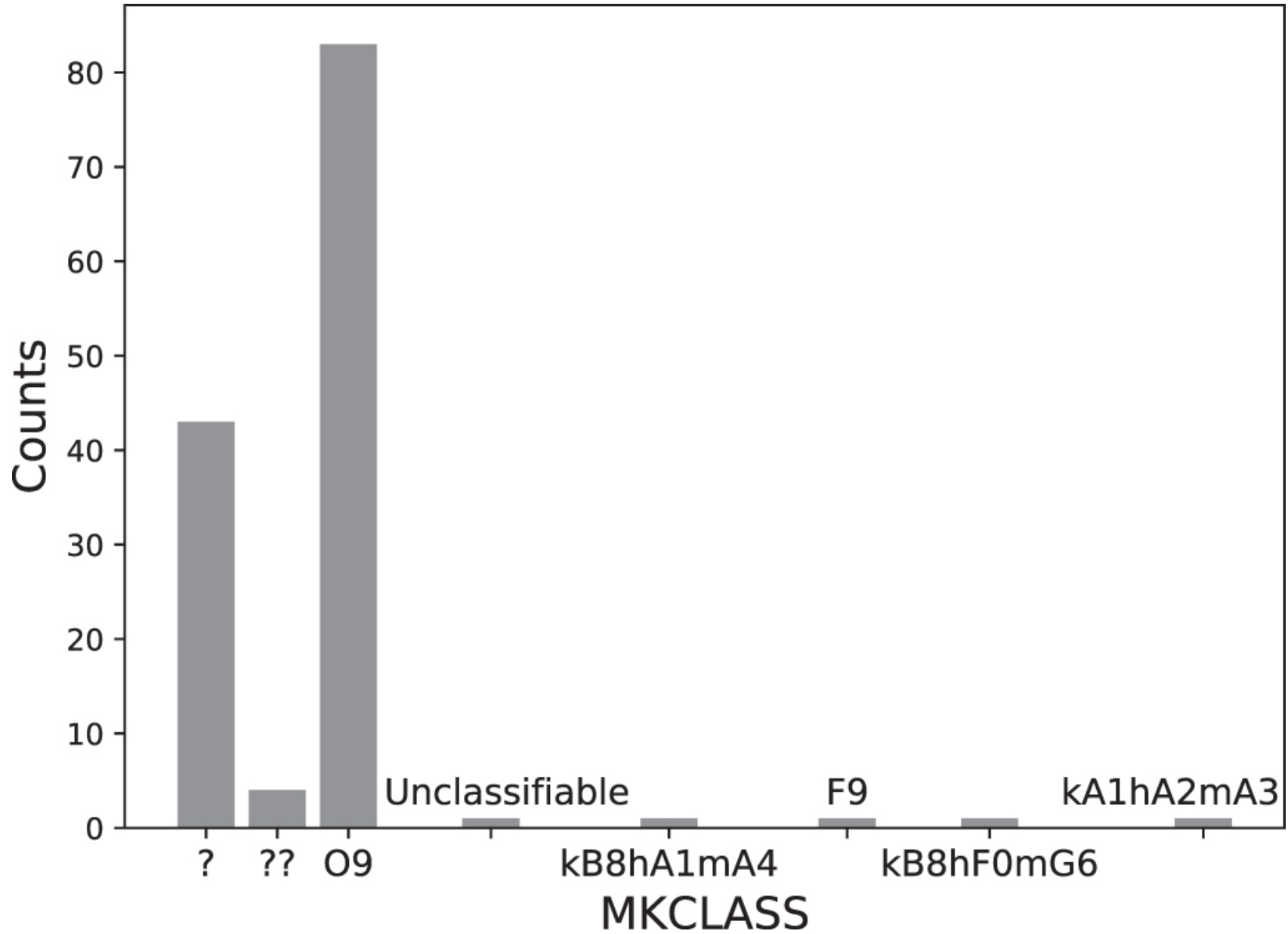
Figure 7. from A Catalog of OB Stars from LAMOST Spectroscopic Survey null 2019 APJS 241 32 doi:10.3847/1538-4365/ab0a0d http://dx.doi.org/10.3847/1538-4365/ab0a0d © 2019. The American Astronomical Society. All rights reserved.
