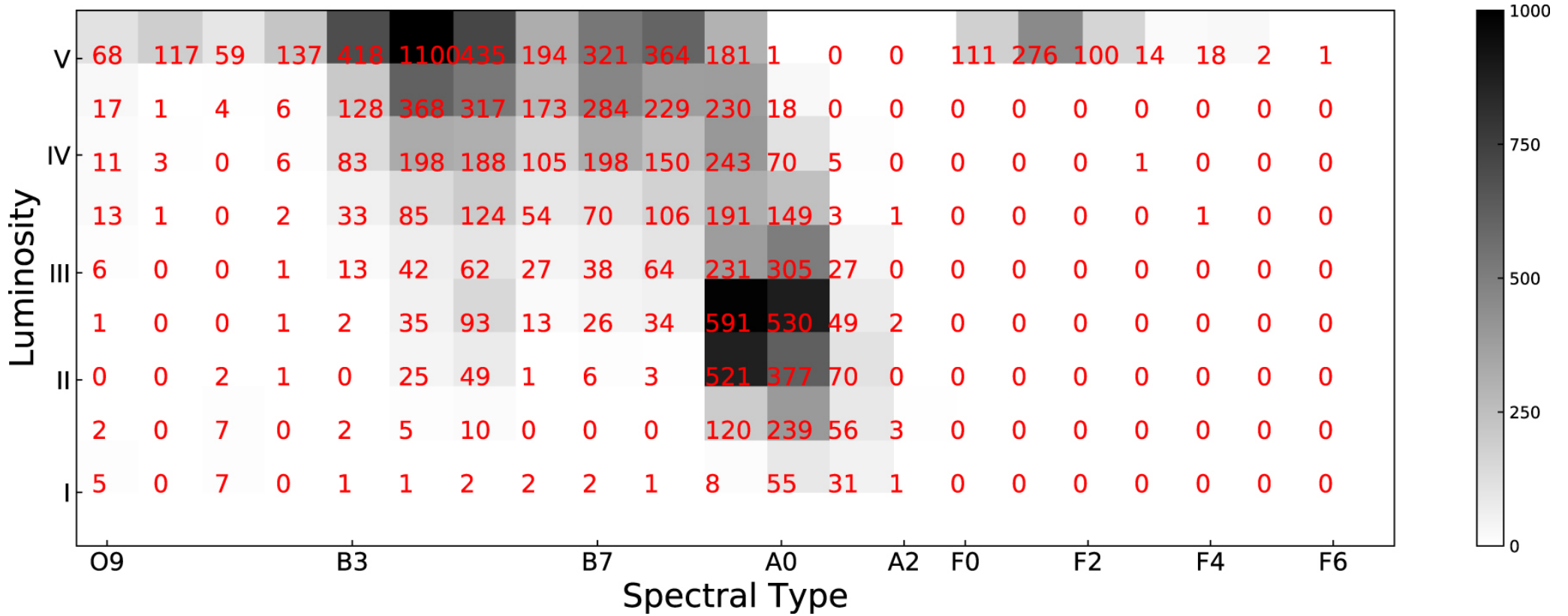
Figure 6. from A Catalog of OB Stars from LAMOST Spectroscopic Survey null 2019 APJS 241 32 doi:10.3847/1538-4365/ab0a0d http://dx.doi.org/10.3847/1538-4365/ab0a0d © 2019. The American Astronomical Society. All rights reserved.
