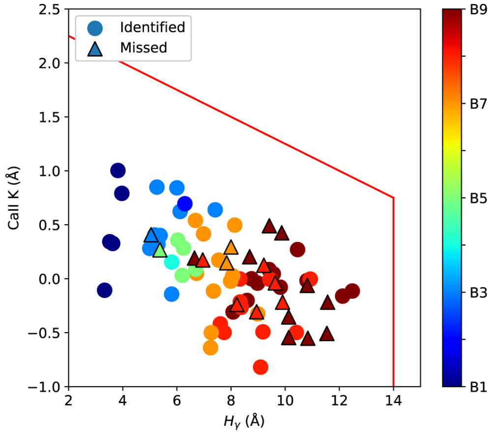
Figure 4. from A Catalog of OB Stars from LAMOST Spectroscopic Survey null 2019 APJS 241 32 doi:10.3847/1538-4365/ab0a0d http://dx.doi.org/10.3847/1538-4365/ab0a0d © 2019. The American Astronomical Society. All rights reserved.
