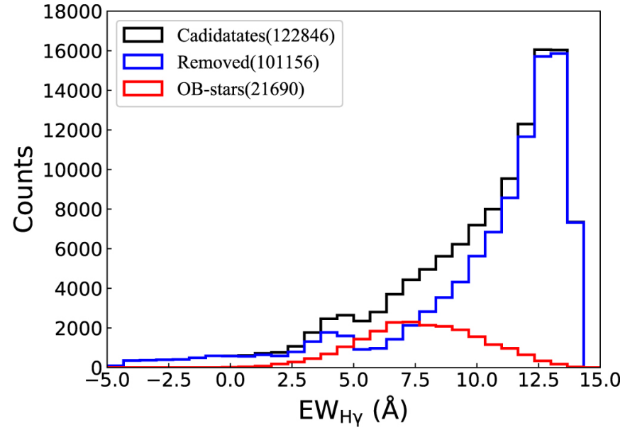
Figure 3. from A Catalog of OB Stars from LAMOST Spectroscopic Survey null 2019 APJS 241 32 doi:10.3847/1538-4365/ab0a0d http://dx.doi.org/10.3847/1538-4365/ab0a0d
