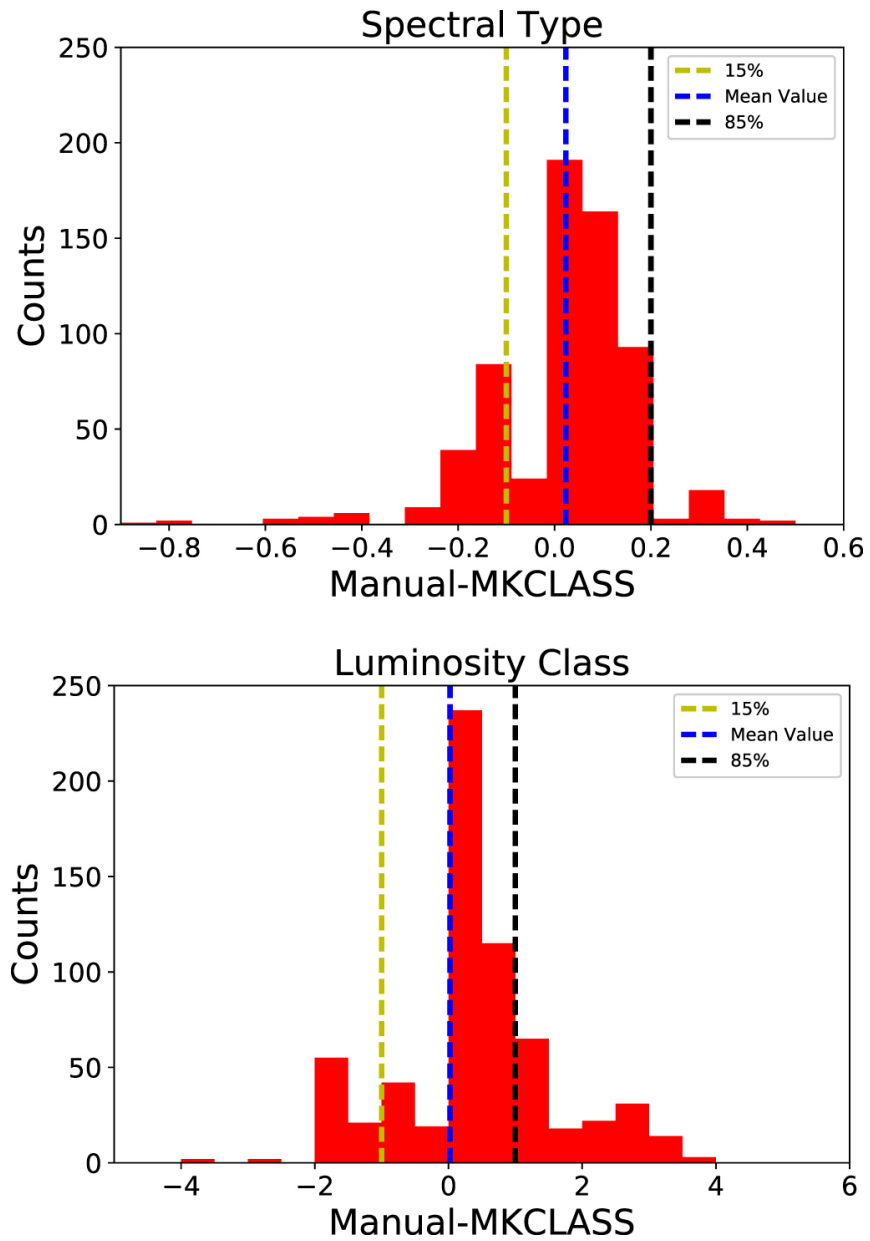
Figure 14. from A Catalog of OB Stars from LAMOST Spectroscopic Survey null 2019 APJS 241 32 doi:10.3847/1538-4365/ab0a0d http://dx.doi.org/10.3847/1538-4365/ab0a0d © 2019. The American Astronomical Society. All rights reserved.
