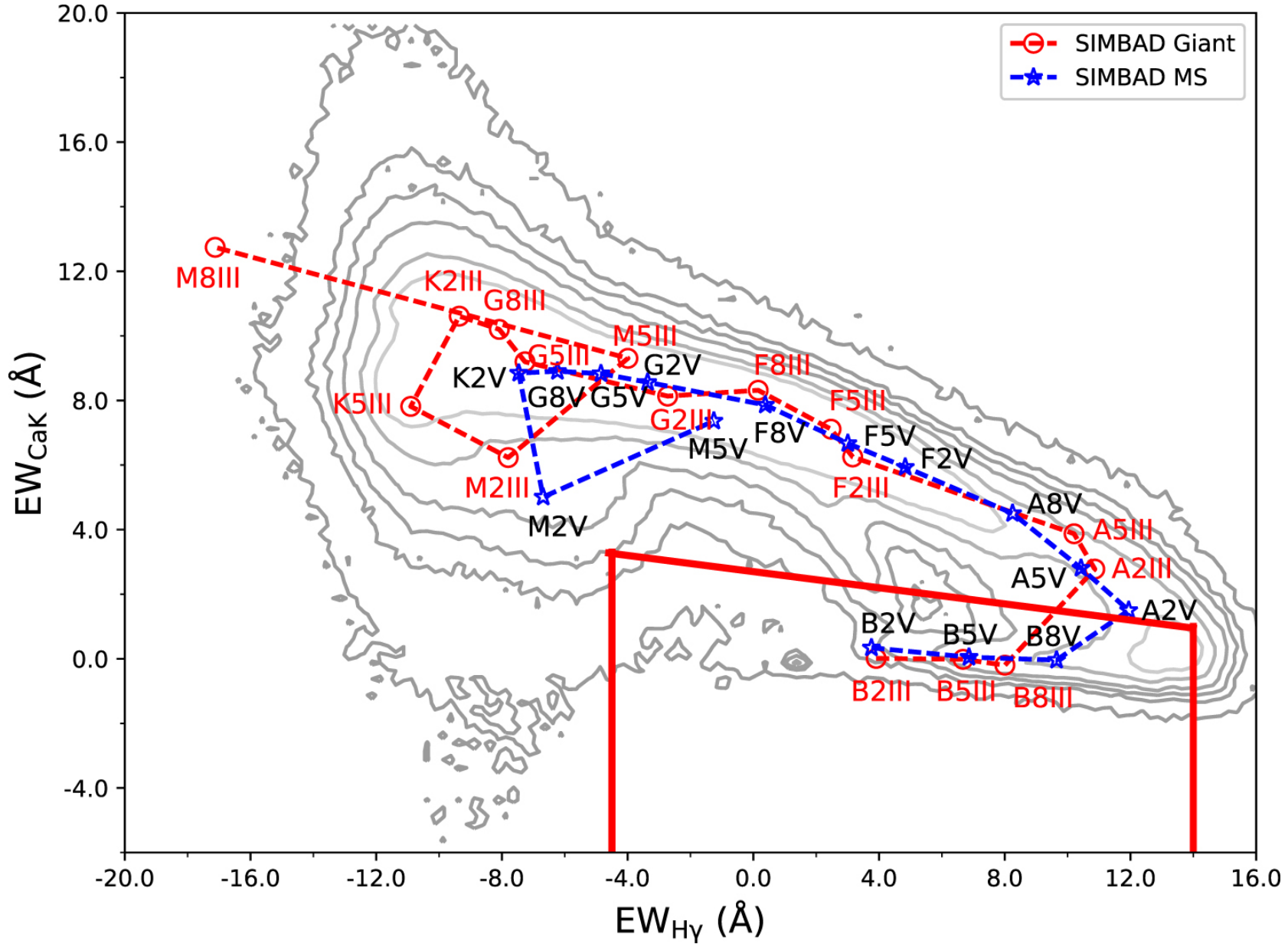
Figure 1. from A Catalog of OB Stars from LAMOST Spectroscopic Survey null 2019 APJS 241 32 doi:10.3847/1538-4365/ab0a0d http://dx.doi.org/10.3847/1538-4365/ab0a0d © 2019. The American Astronomical Society. All rights reserved.
