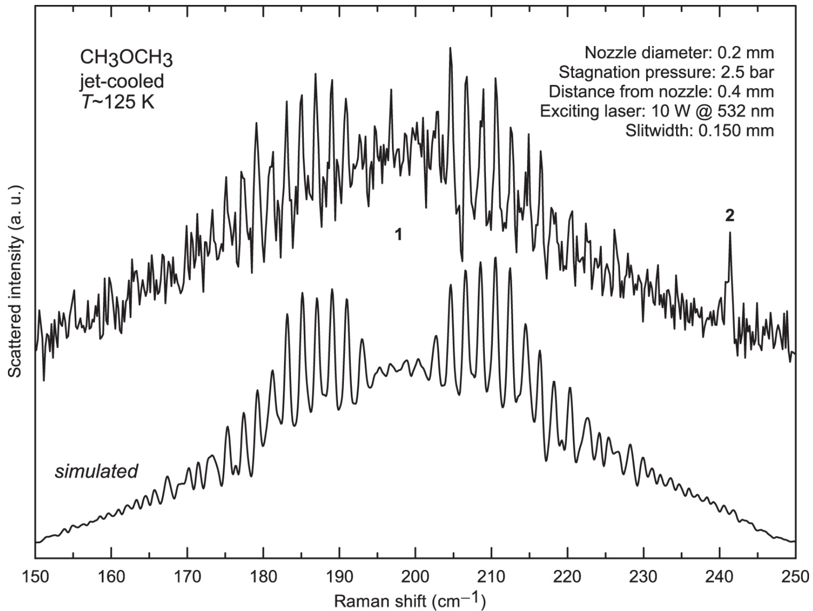
Figure 2. from New Spectral Characterization of Dimethyl Ether Isotopologues CH 3 OCH 3 and 13 CH 3 OCH 3 in the THz Region null 2019 APJS 241 13 doi:10.3847/1538-4365/ab041e http://dx.doi.org/10.3847/1538-4365/ab041e © 2019. The American Astronomical Society. All rights reserved.
