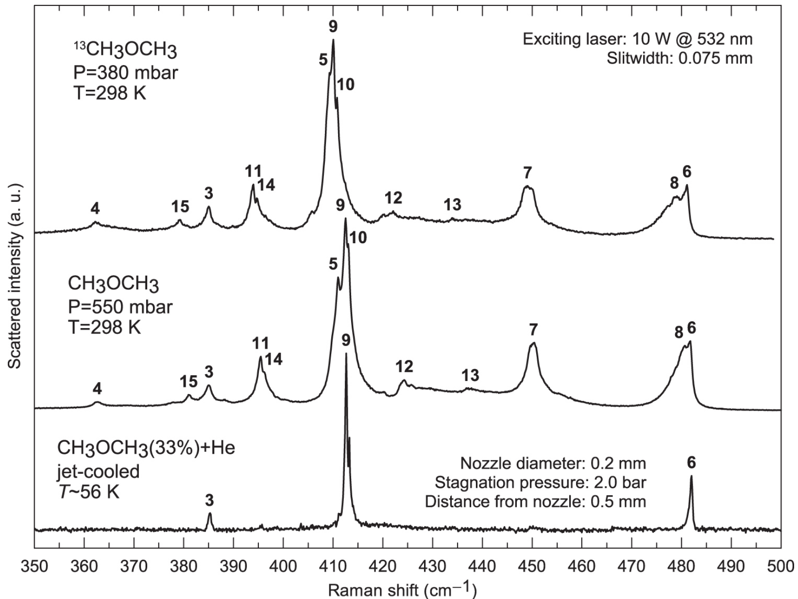
Figure 1. from New Spectral Characterization of Dimethyl Ether Isotopologues CH 3 OCH 3 and 13 CH 3 OCH 3 in the THz Region null 2019 APJS 241 13 doi:10.3847/1538-4365/ab041e http://dx.doi.org/10.3847/1538-4365/ab041e © 2019. The American Astronomical Society. All rights reserved.
