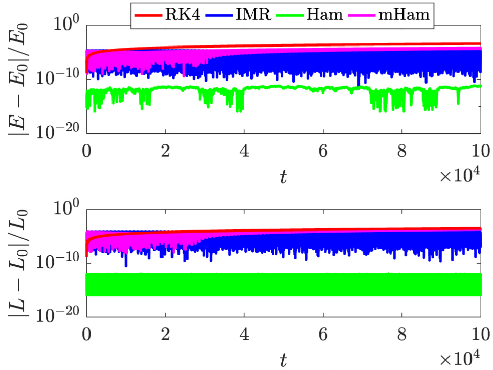
(a) E = 0.885, L = -7 regular orbit.
