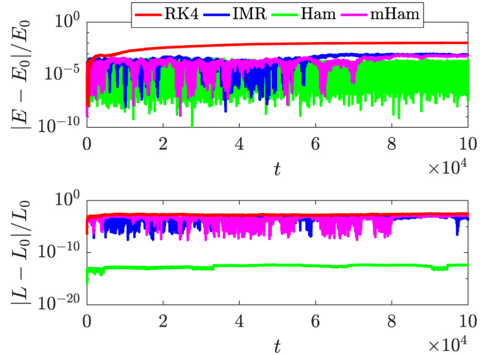
(b) E = 0.89, L = -7 chaotic orbit.
