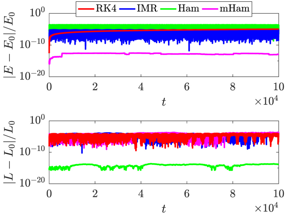
(a) Regular orbit RSA5.
