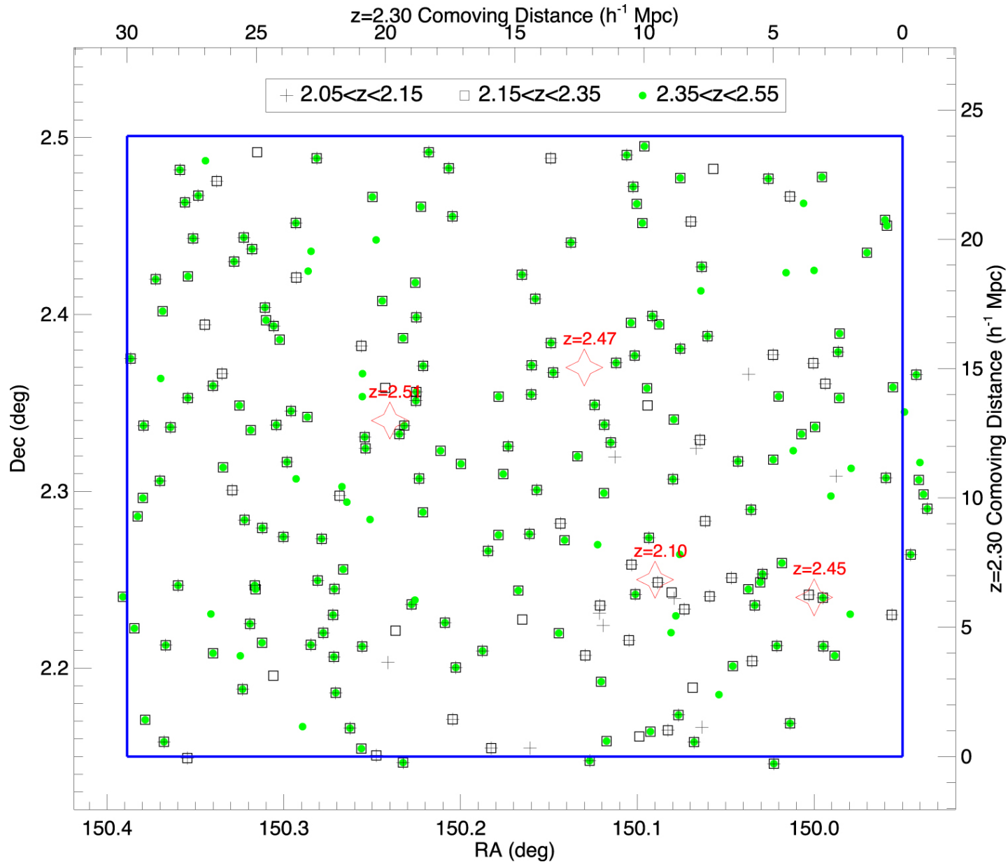
Figure 6. from First Data Release of the COSMOS Ly Mapping and Tomography Observations: 3D Ly Forest Tomography at 2.05 < z < 2.55 null 2018 APJS 237 31 doi:10.3847/1538-4365/aace58 https://dx.doi.org/10.3847/1538-4365/aace58 © 2018. The American Astronomical Society. All rights reserved.
