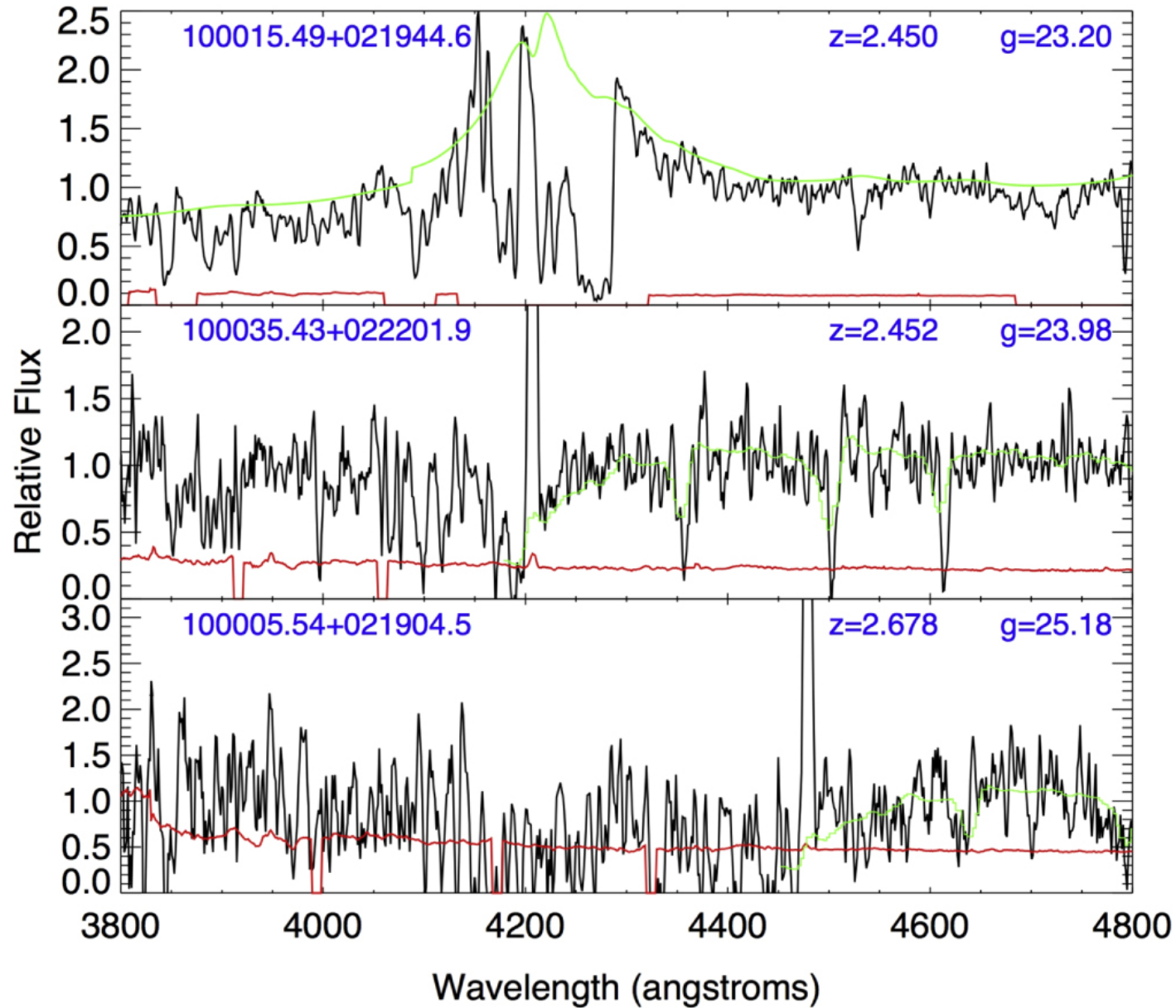
Figure 5. from First Data Release of the COSMOS Ly Mapping and Tomography Observations: 3D Ly Forest Tomography at 2.05 < z < 2.55 null 2018 APJS 237 31 doi:10.3847/1538-4365/aace58 https://dx.doi.org/10.3847/1538-4365/aace58 © 2018. The American Astronomical Society. All rights reserved.
