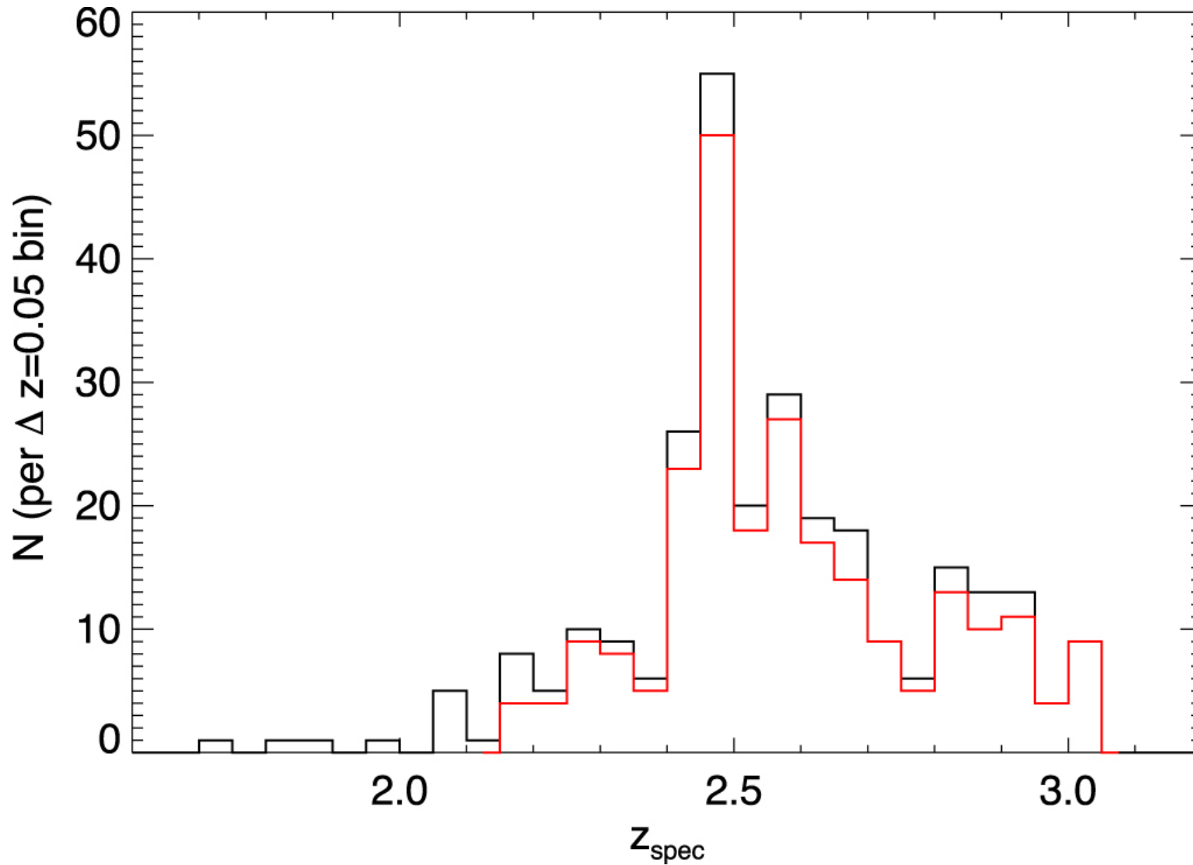
Figure 4. from First Data Release of the COSMOS Ly Mapping and Tomography Observations: 3D Ly Forest Tomography at 2.05 < z < 2.55 null 2018 APJS 237 31 doi:10.3847/1538-4365/aace58 https://dx.doi.org/10.3847/1538-4365/aace58 © 2018. The American Astronomical Society. All rights reserved.
