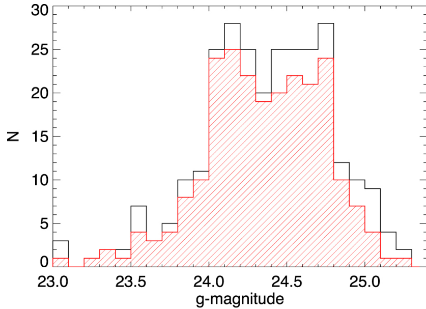
Figure 3. from First Data Release of the COSMOS Ly Mapping and Tomography Observations: 3D Ly Forest Tomography at 2.05 < z < 2.55 null 2018 APJS 237 31 doi:10.3847/1538-4365/aace58 https://dx.doi.org/10.3847/1538-4365/aace58 © 2018. The American Astronomical Society. All rights reserved.
