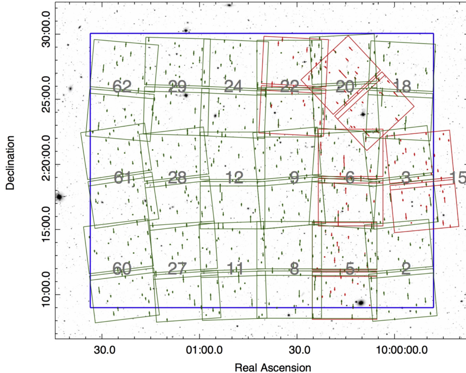
Figure 2. from First Data Release of the COSMOS Ly Mapping and Tomography Observations: 3D Ly Forest Tomography at 2.05 < z < 2.55 null 2018 APJS 237 31 doi:10.3847/1538-4365/aace58 https://dx.doi.org/10.3847/1538-4365/aace58 © 2018. The American Astronomical Society. All rights reserved.
