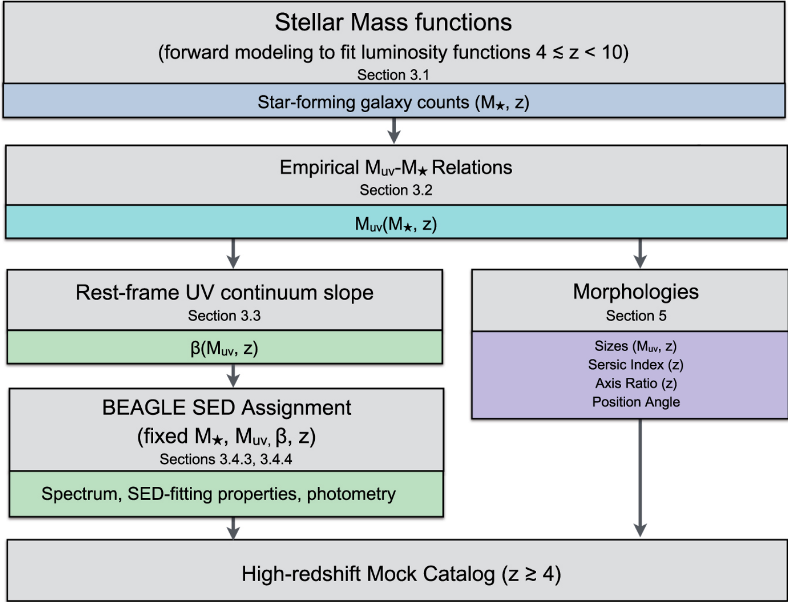
Figure 2. from The JWST Extragalactic Mock Catalog: Modeling Galaxy Populations from the UV through the Near-IR over 13 Billion Years of Cosmic History null 2018 APJS 236 33 doi:10.3847/1538-4365/aabcbb https://dx.doi.org/10.3847/1538-4365/aabcbb © 2018. The American Astronomical Society. All rights reserved.
