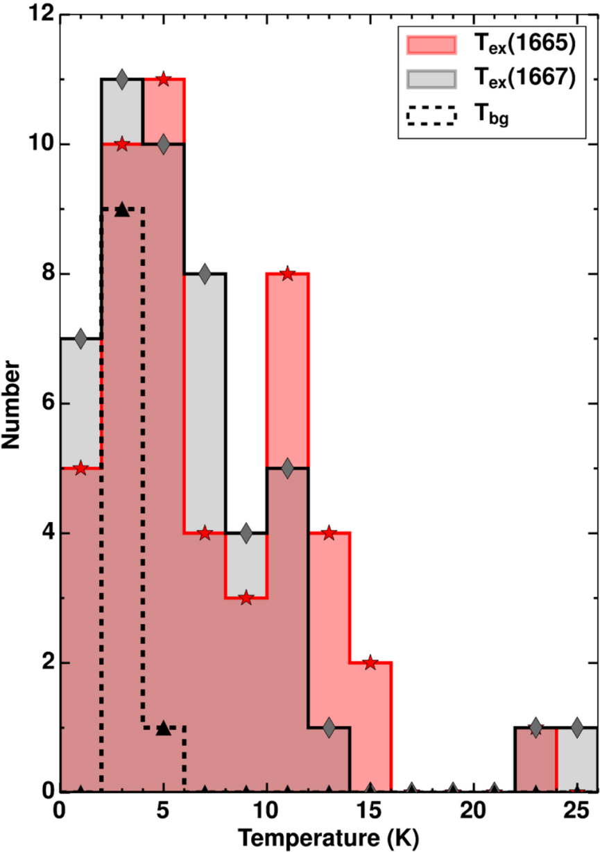
Figure 5. from Where is OH and Does It Trace the Dark Molecular Gas (DMG)? null 2018 APJS 235 1 doi:10.3847/1538-4365/aaa762 https://dx.doi.org/10.3847/1538-4365/aaa762 © 2018. The American Astronomical Society. All rights reserved.
