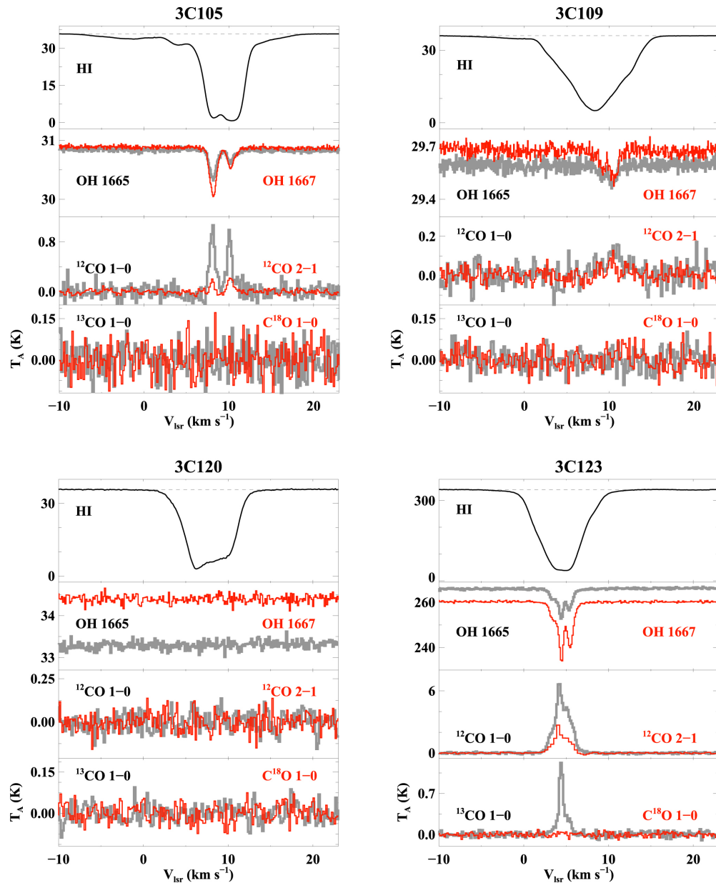
Figure 13. Spectra of H I, OH, and CO toward continuum sources from Where is OH and Does It Trace the Dark Molecular Gas (DMG)? null 2018 APJS 235 1 doi:10.3847/1538-4365/aaa762 https://dx.doi.org/10.3847/1538-4365/aaa762 © 2018. The American Astronomical Society. All rights reserved.
