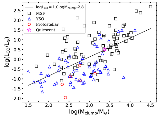
Figure 9. from Massive Outflows Associated with ATLASGAL Clumps null 2018 APJS 235 3 doi:10.3847/1538-4365/aaa297 https://dx.doi.org/10.3847/1538-4365/aaa297 © 2018. The American Astronomical Society. All rights reserved.
