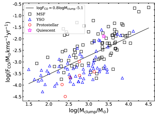
Figure 8. from Massive Outflows Associated with ATLASGAL Clumps null 2018 APJS 235 3 doi:10.3847/1538-4365/aaa297 https://dx.doi.org/10.3847/1538-4365/aaa297 © 2018. The American Astronomical Society. All rights reserved.
