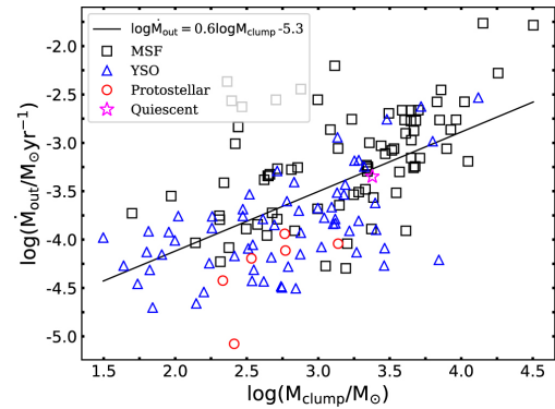
Figure 7. from Massive Outflows Associated with ATLASGAL Clumps null 2018 APJS 235 3 doi:10.3847/1538-4365/aaa297 https://dx.doi.org/10.3847/1538-4365/aaa297 © 2018. The American Astronomical Society. All rights reserved.
