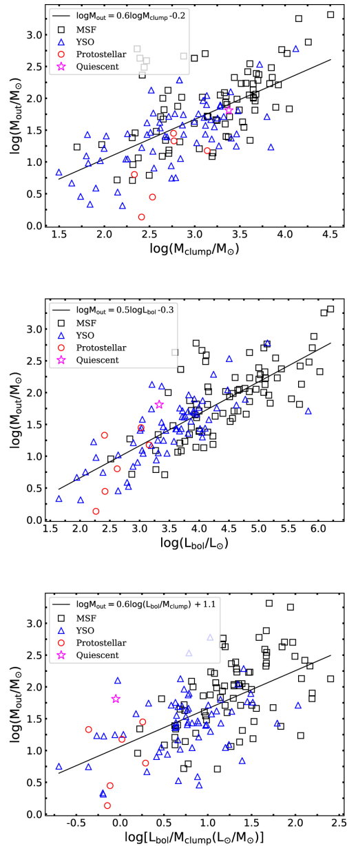
Figure 6. from Massive Outflows Associated with ATLASGAL Clumps null 2018 APJS 235 3 doi:10.3847/1538-4365/aaa297 https://dx.doi.org/10.3847/1538-4365/aaa297 © 2018. The American Astronomical Society. All rights reserved.
