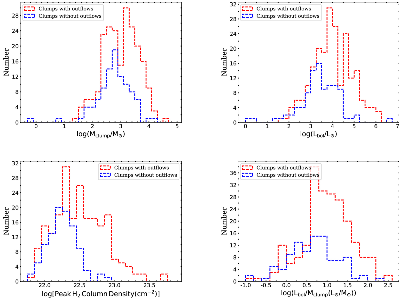
Figure 5. from Massive Outflows Associated with ATLASGAL Clumps null 2018 APJS 235 3 doi:10.3847/1538-4365/aaa297 https://dx.doi.org/10.3847/1538-4365/aaa297 © 2018. The American Astronomical Society. All rights reserved.
