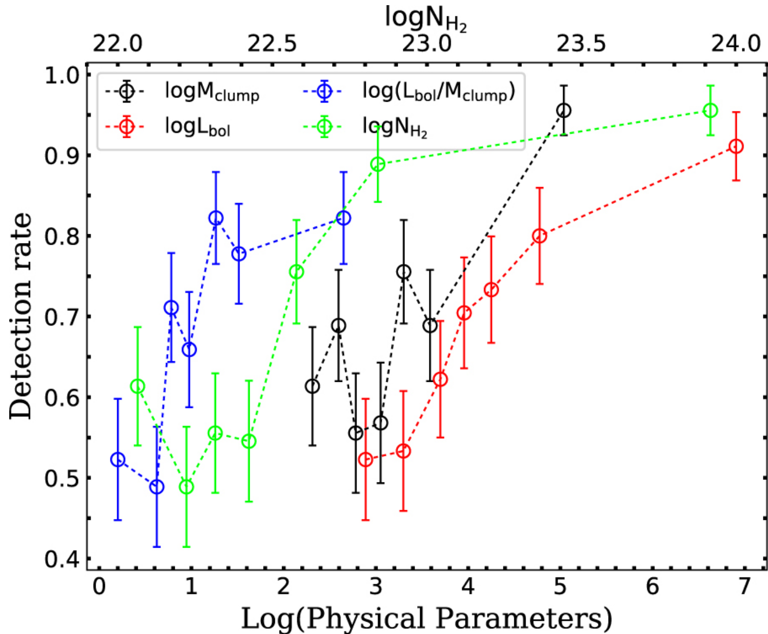
Figure 4. from Massive Outflows Associated with ATLASGAL Clumps null 2018 APJS 235 3 doi:10.3847/1538-4365/aaa297 https://dx.doi.org/10.3847/1538-4365/aaa297 © 2018. The American Astronomical Society. All rights reserved.
