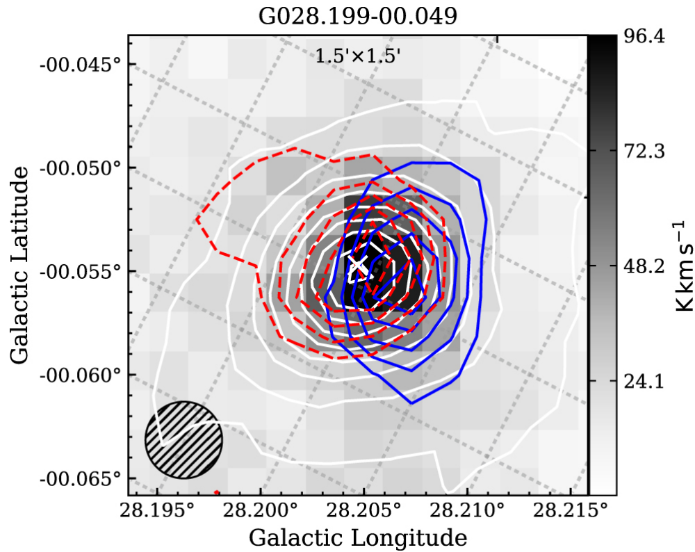
Figure 3. from Massive Outflows Associated with ATLASGAL Clumps null 2018 APJS 235 3 doi:10.3847/1538-4365/aaa297 https://dx.doi.org/10.3847/1538-4365/aaa297 © 2018. The American Astronomical Society. All rights reserved.
