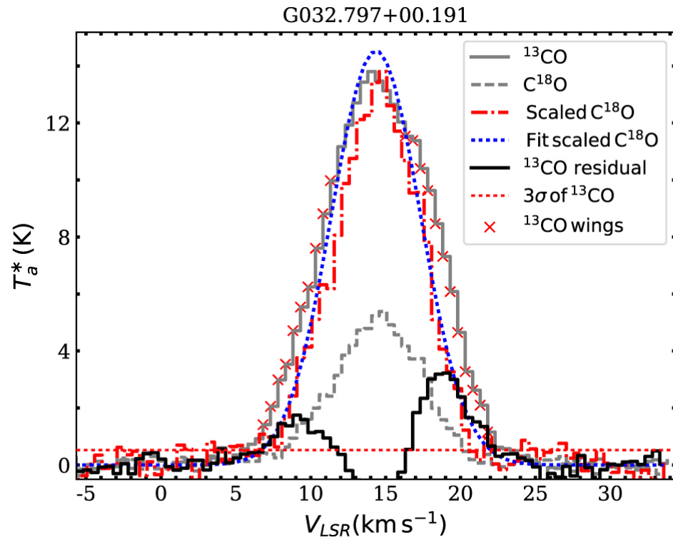
Figure 2. from Massive Outflows Associated with ATLASGAL Clumps null 2018 APJS 235 3 doi:10.3847/1538-4365/aaa297 https://dx.doi.org/10.3847/1538-4365/aaa297 © 2018. The American Astronomical Society. All rights reserved.
