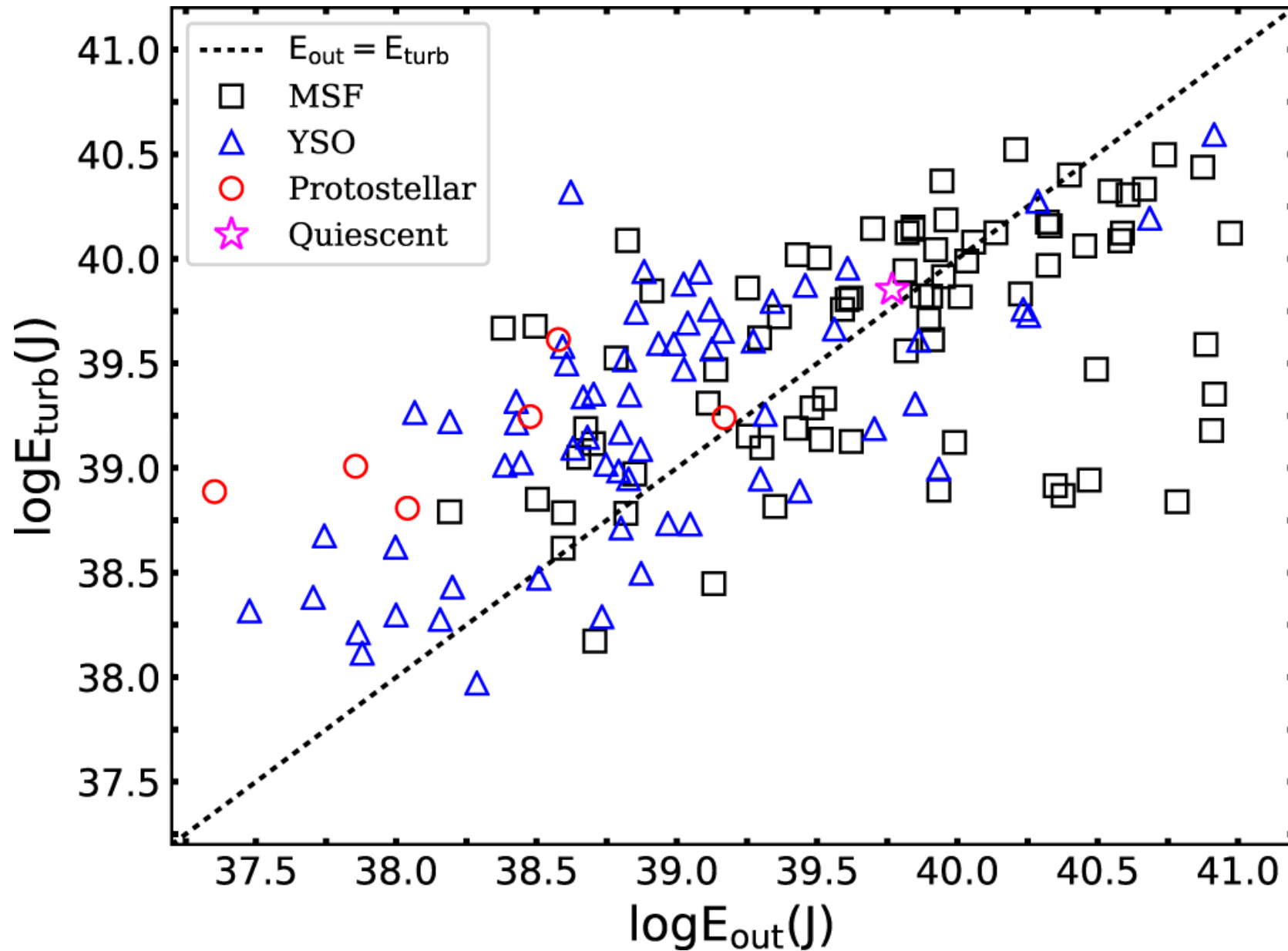
Figure 11. from Massive Outflows Associated with ATLASGAL Clumps null 2018 APJS 235 3 doi:10.3847/1538-4365/aaa297 https://dx.doi.org/10.3847/1538-4365/aaa297 © 2018. The American Astronomical Society. All rights reserved.
