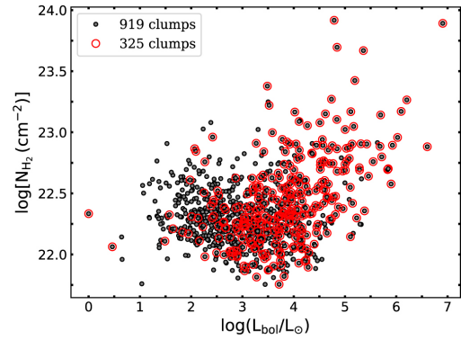
Figure 1. from Massive Outflows Associated with ATLASGAL Clumps null 2018 APJS 235 3 doi:10.3847/1538-4365/aaa297 https://dx.doi.org/10.3847/1538-4365/aaa297 © 2018. The American Astronomical Society. All rights reserved.
