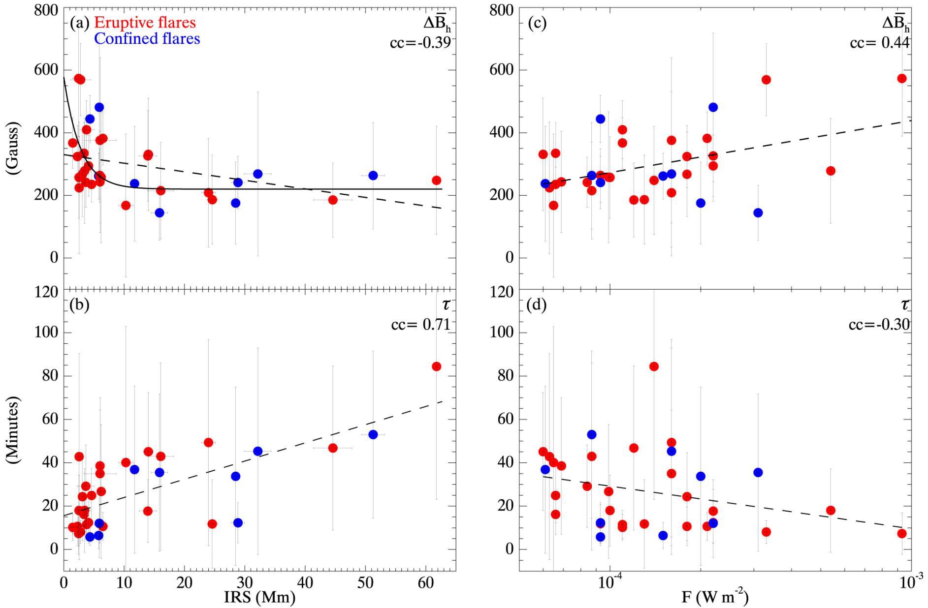
Figure 5. from Lijuan Liu et al 2022 Astrophys. J. Lett. 934 doi:10.3847/2041-8213/ac83bf http://dx.doi.org/10.3847/2041-8213/ac83bf © 2022. The Author(s). Published by the American Astronomical Society.
