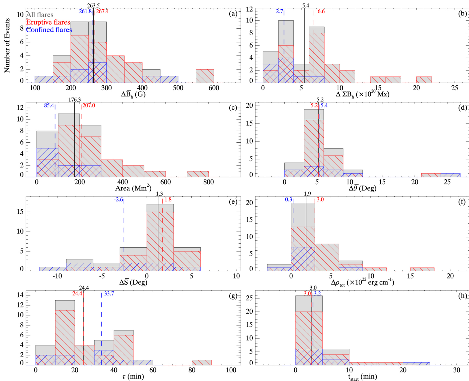
Figure 3. from Lijuan Liu et al 2022 Astrophys. J. Lett. 934 doi:10.3847/2041-8213/ac83bf https://dx.doi.org/10.3847/2041-8213/ac83bf © 2022. The Author(s). Published by the American Astronomical Society.
