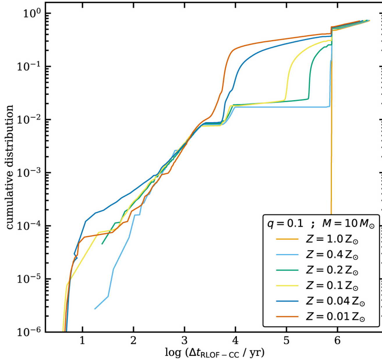
Figure 8. from Alexandra Kozyreva et al 2022 Astrophys. J. Lett. 934 doi:10.3847/2041-8213/ac835a http://dx.doi.org/10.3847/2041-8213/ac835a © 2022. The Author(s). Published by the American Astronomical Society.
