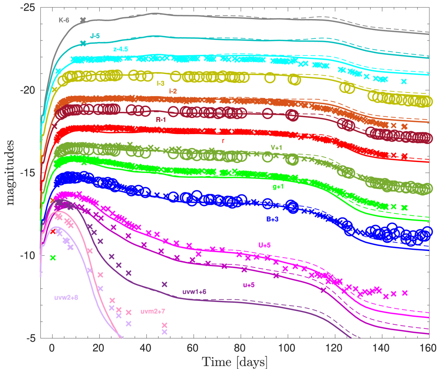
Figure 4. from Alexandra Kozyreva et al 2022 Astrophys. J. Lett. 934 doi:10.3847/2041-8213/ac835a https://dx.doi.org/10.3847/2041-8213/ac835a © 2022. The Author(s). Published by the American Astronomical Society.
