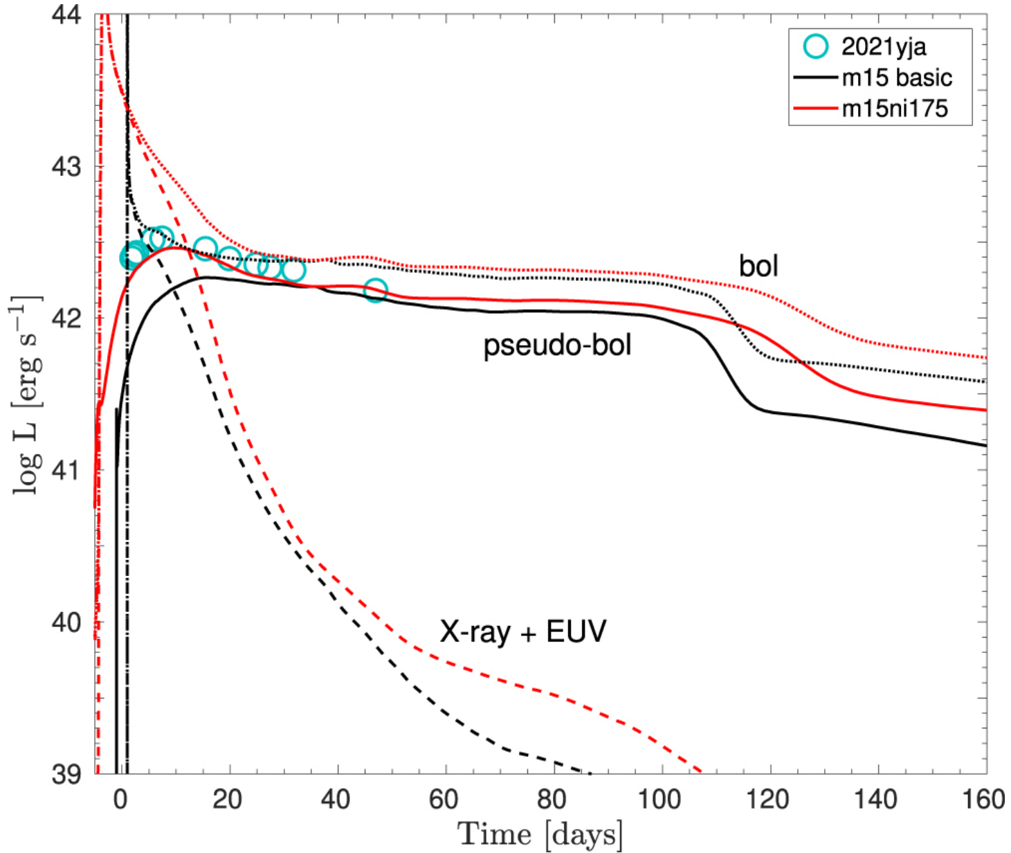
Figure 3. from Alexandra Kozyreva et al 2022 Astrophys. J. Lett. 934 doi:10.3847/2041-8213/ac835a http://dx.doi.org/10.3847/2041-8213/ac835a © 2022. The Author(s). Published by the American Astronomical Society.
