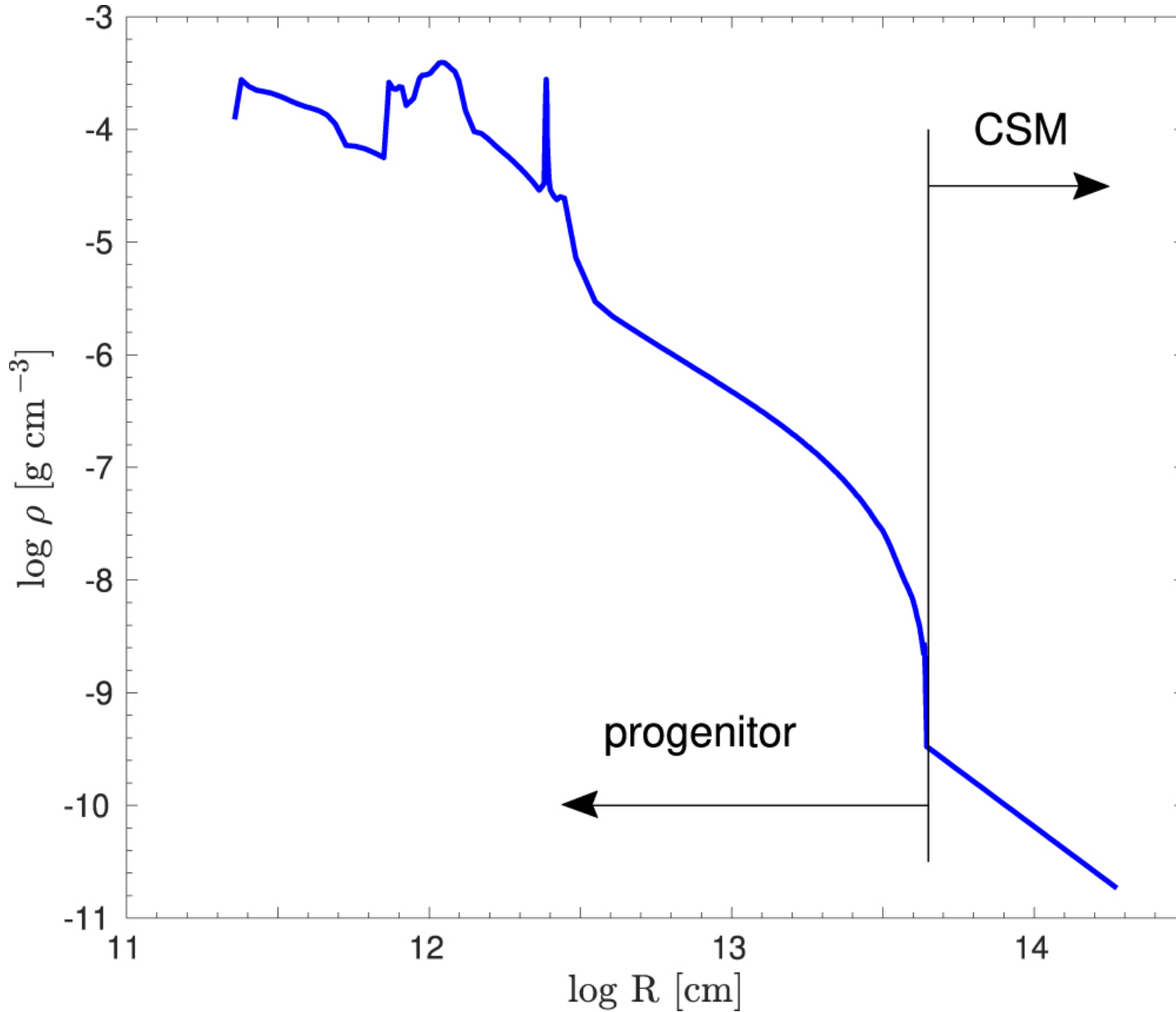
Figure 2. from Alexandra Kozyreva et al 2022 Astrophys. J. Lett. 934 doi:10.3847/2041-8213/ac835a http://dx.doi.org/10.3847/2041-8213/ac835a © 2022. The Author(s). Published by the American Astronomical Society.
