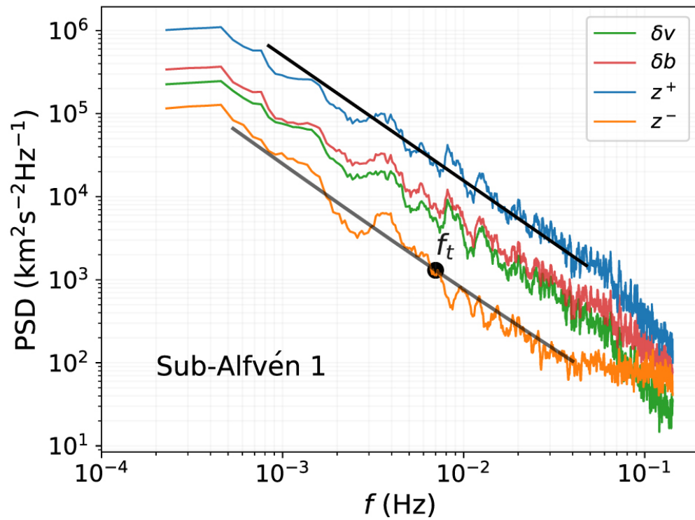
Figure 3. from L.-L. Zhao et al 2022 Astrophys. J. Lett. 934 doi:10.3847/2041-8213/ac8353 http://dx.doi.org/10.3847/2041-8213/ac8353 © 2022. The Author(s). Published by the American Astronomical Society.
