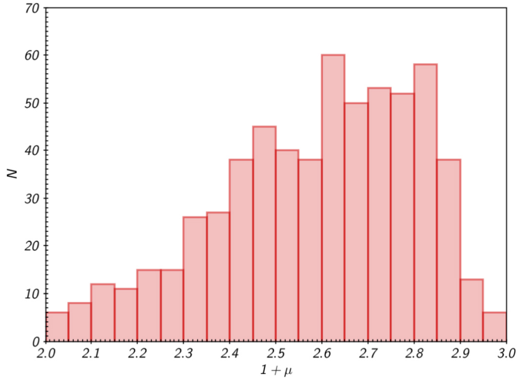
Figure 2. from High-frequency Magnetic Fluctuations in Space Plasmas and the Role of Electron Landau Damping null 2022 APJL 924 L26 doi:10.3847/2041-8213/ac4740 http://dx.doi.org/10.3847/2041-8213/ac4740
