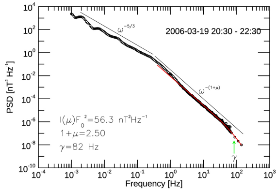
Figure 1. from High-frequency Magnetic Fluctuations in Space Plasmas and the Role of Electron Landau Damping null 2022 APJL 924 L26 doi:10.3847/2041-8213/ac4740 http://dx.doi.org/10.3847/2041-8213/ac4740
