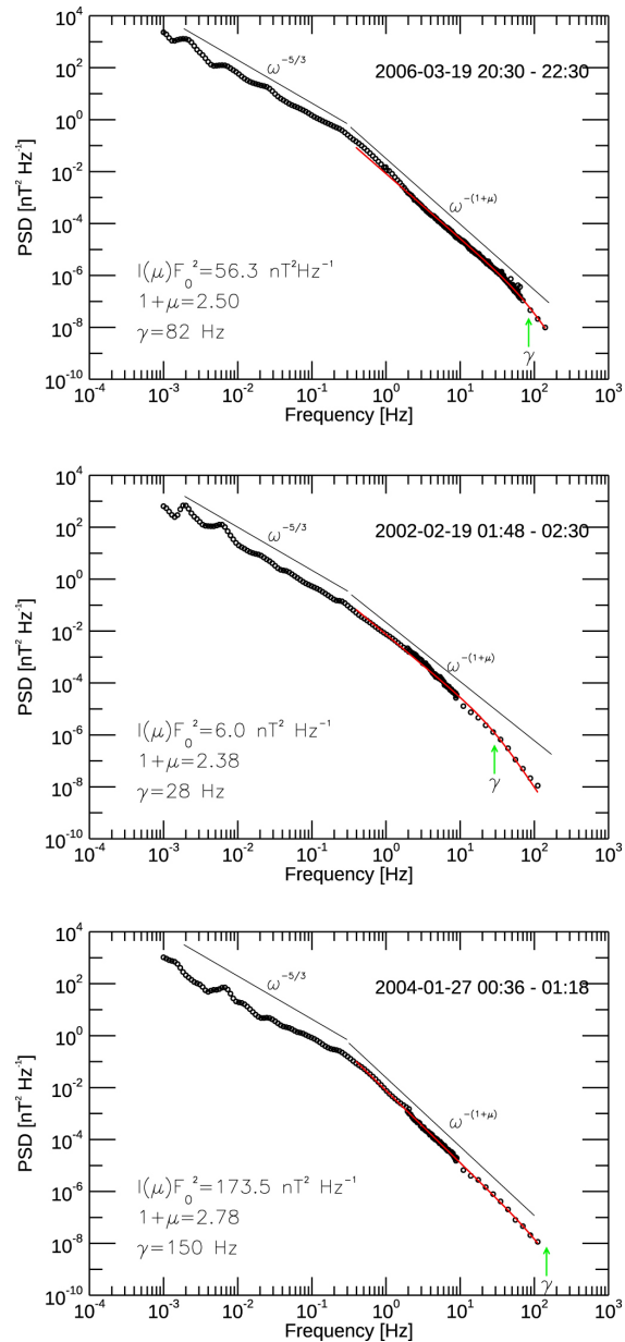
Figure 1. from High-frequency Magnetic Fluctuations in Space Plasmas and the Role of Electron Landau Damping null 2022 APJL 924 L26 doi:10.3847/2041-8213/ac4740 https://dx.doi.org/10.3847/2041-8213/ac4740 © 2022. The Author(s). Published by the American Astronomical Society.
