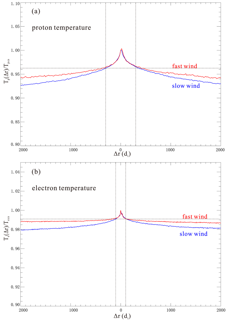
Figure 2. from Evidence for Plasma Heating at Thin Current Sheets in the Solar Wind null 2022 APJL 924 L22 doi:10.3847/2041-8213/ac4701 https://dx.doi.org/10.3847/2041-8213/ac4701 © 2022. The Author(s). Published by the American Astronomical Society.
