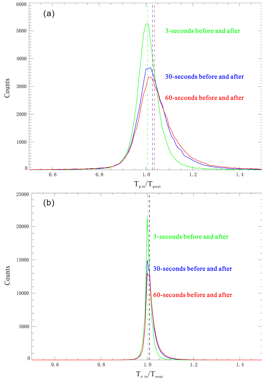
Figure 1. from Evidence for Plasma Heating at Thin Current Sheets in the Solar Wind null 2022 APJL 924 L22 doi:10.3847/2041-8213/ac4701 https://dx.doi.org/10.3847/2041-8213/ac4701 © 2022. The Author(s). Published by the American Astronomical Society.
