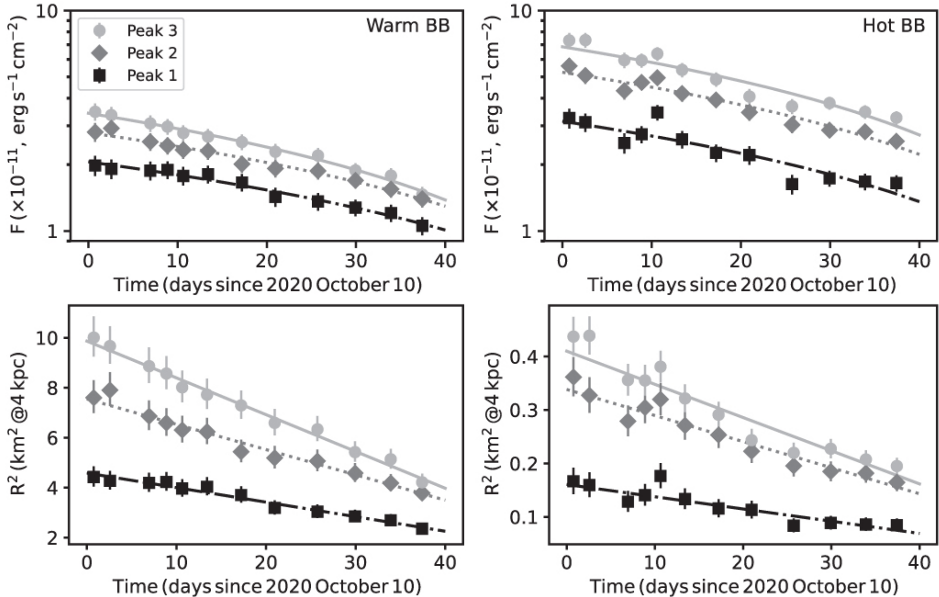
Figure 5. from Pulse Peak Migration during the Outburst Decay of the Magnetar SGR 1830-0645: Crustal Motion and Magnetospheric Untwisting null 2022 APJL 924 L27 doi:10.3847/2041-8213/ac4700 http://dx.doi.org/10.3847/2041-8213/ac4700 © 2022. The Author(s). Published by the American Astronomical Society.
