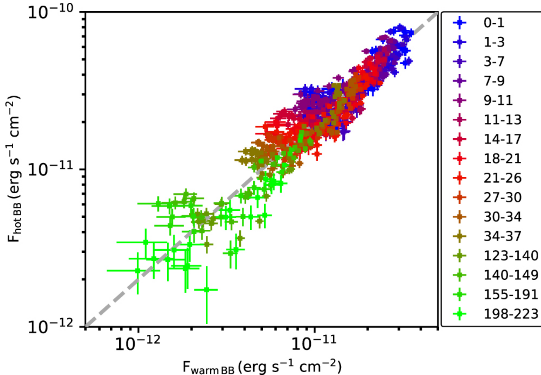
Figure 4. from Pulse Peak Migration during the Outburst Decay of the Magnetar SGR 1830-0645: Crustal Motion and Magnetospheric Untwisting null 2022 APJL 924 L27 doi:10.3847/2041-8213/ac4700 https://dx.doi.org/10.3847/2041-8213/ac4700 © 2022. The Author(s). Published by the American Astronomical Society.
