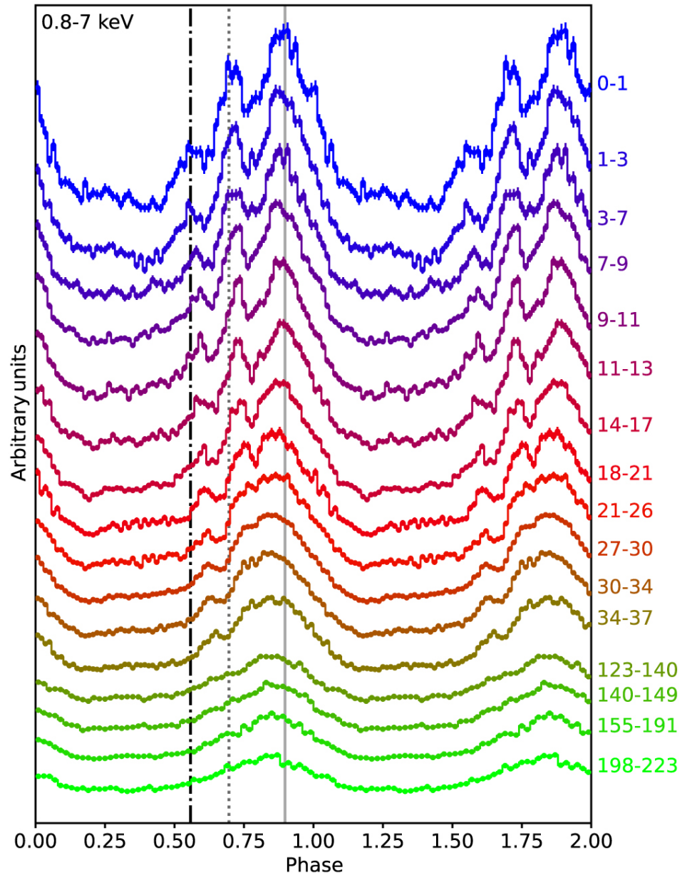
Figure 1. from Pulse Peak Migration during the Outburst Decay of the Magnetar SGR 1830-0645: Crustal Motion and Magnetospheric Untwisting null 2022 APJL 924 L27 doi:10.3847/2041-8213/ac4700 http://dx.doi.org/10.3847/2041-8213/ac4700 © 2022. The Author(s). Published by the American Astronomical Society.
