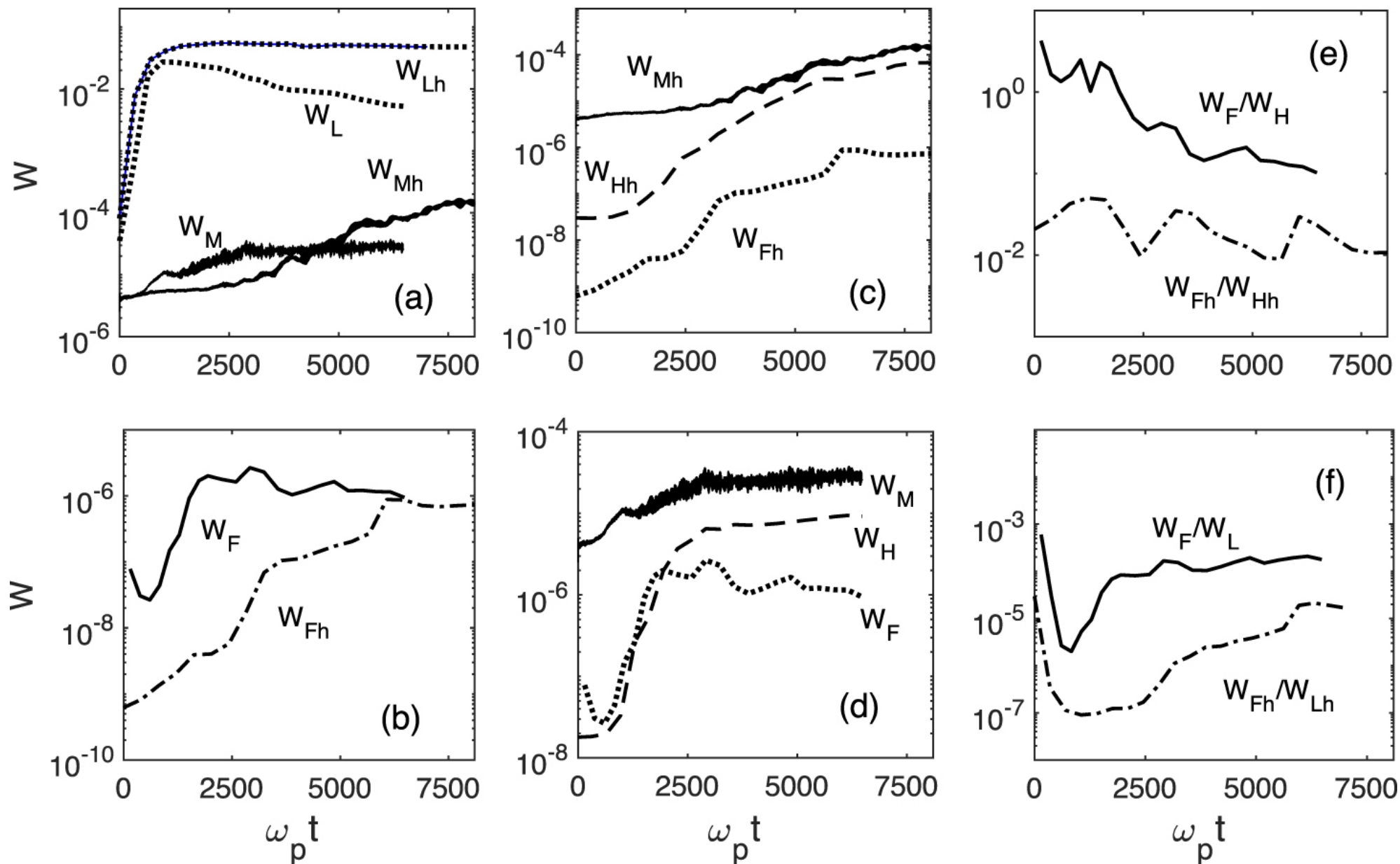
Figure 5. from Fundamental Electromagnetic Emissions by a Weak Electron Beam in Solar Wind Plasmas with Density Fluctuations null 2022 APJL 924 L24 doi:10.3847/2041-8213/ac46a7 https://dx.doi.org/10.3847/2041-8213/ac46a7 © 2022. The Author(s). Published by the American Astronomical Society.
